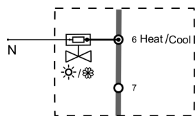
Figure 2 2-pipe wiring
