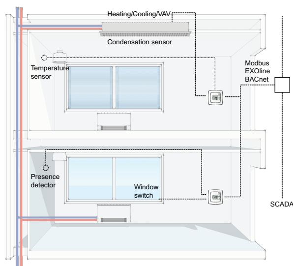
Fig. 1 Room installation example
