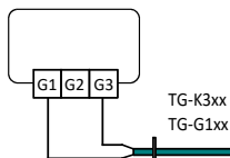
Fig. 2 External sensor and internal setpoint
