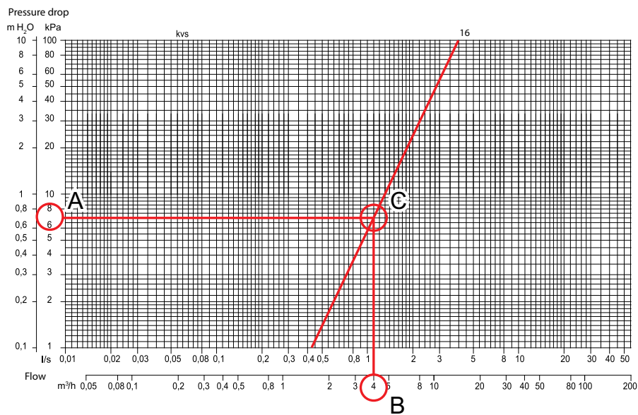
Fig. 3 Example, calculation of kv value: If the pressure drop is 7 kPa (A) and the flow is 4 m³/h (B), the kv value is 16 (C). See the markings in the picture to the right.
