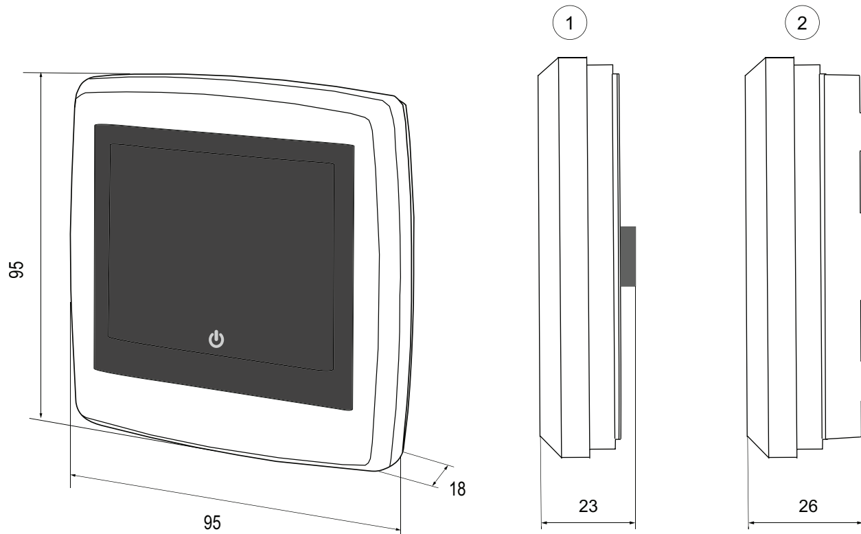
Fig. 11: With back plate for flush mounting (ED-RUD-2-FM) 2: With back plate for wall mounting (ED-RUD-2-WM)
